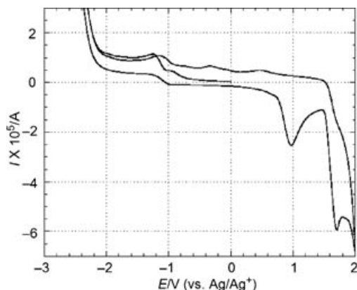
FIGURE 3 Cyclic voltammogram of 6 .
