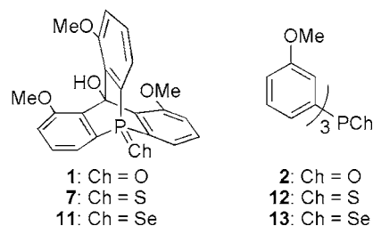
FIGURE 2 The 9-Phosphatriptycene Chalcogenides and Tris(3-methoxyphenyl)phosphine Chalcogenides.
