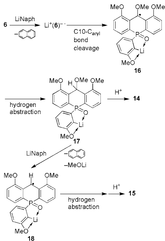
SCHEME 7
