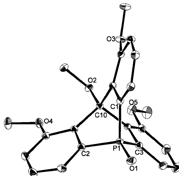
FIGURE 1 ORTEP drawing of 6 (50% probability). Hydrogen atoms and solvent molecules are omitted for clarity. Selected bond lengths ( \text{\AA} ) and angles ( ^\circ ): \text{P}(1)\text{--O}(1) 1.4855(11) , \text{P}(1)\text{--C}(1) 1.7798(13) , \text{P}(1)\text{--C}(2) 1.7714(13) , \text{P}(1)\text{--C}(3) 1.8009(14) , \text{C}(1)\text{--P}(1)\text{--C}(2) 100.32(6) , \text{C}(2)\text{--P}(1)\text{--C}(3) 98.10(6) , \text{C}(1)\text{--P}(1)\text{--C}(3) 99.72(6) .
